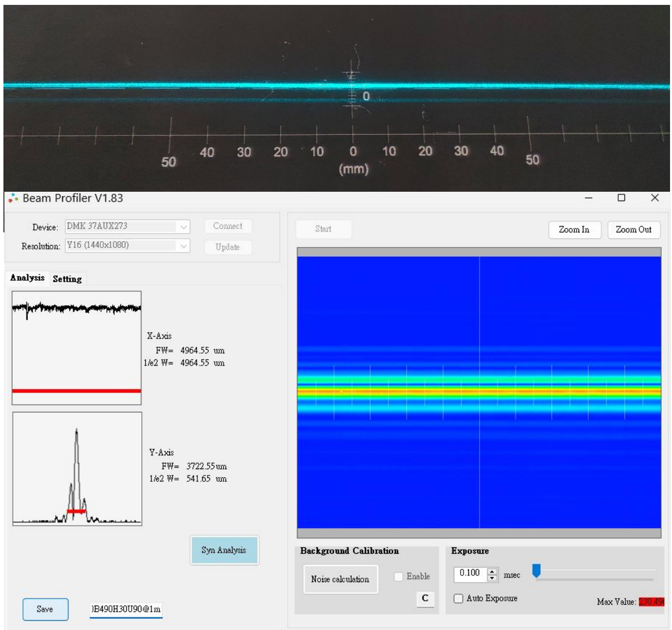
LM10B490H30U90 Line Performance at 1m
